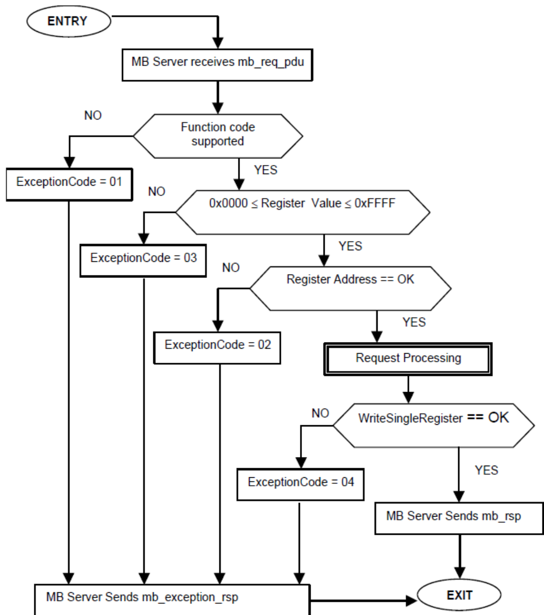
Figure 16: Write Single Register state diagram
