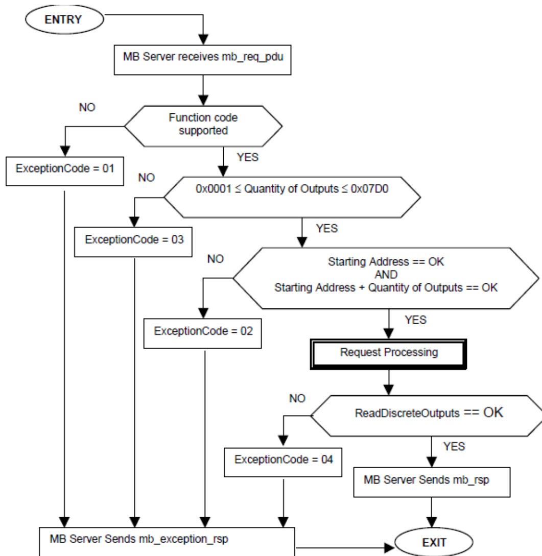
Figure 11: Read Coils state diagram
