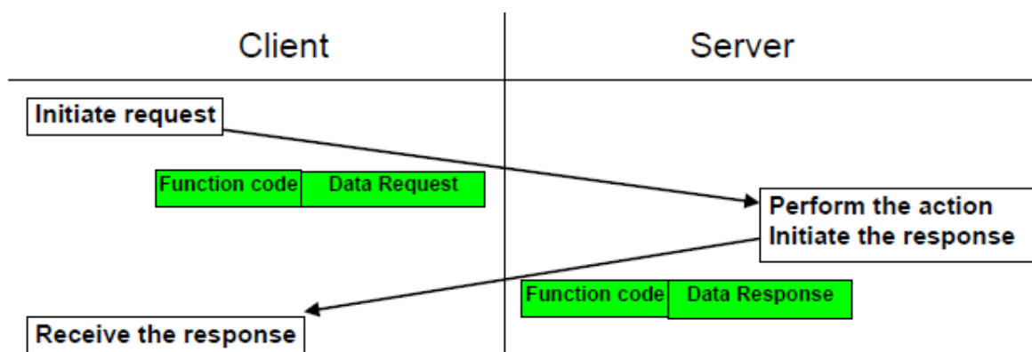
Figure 4: MODBUS transaction (error free)
