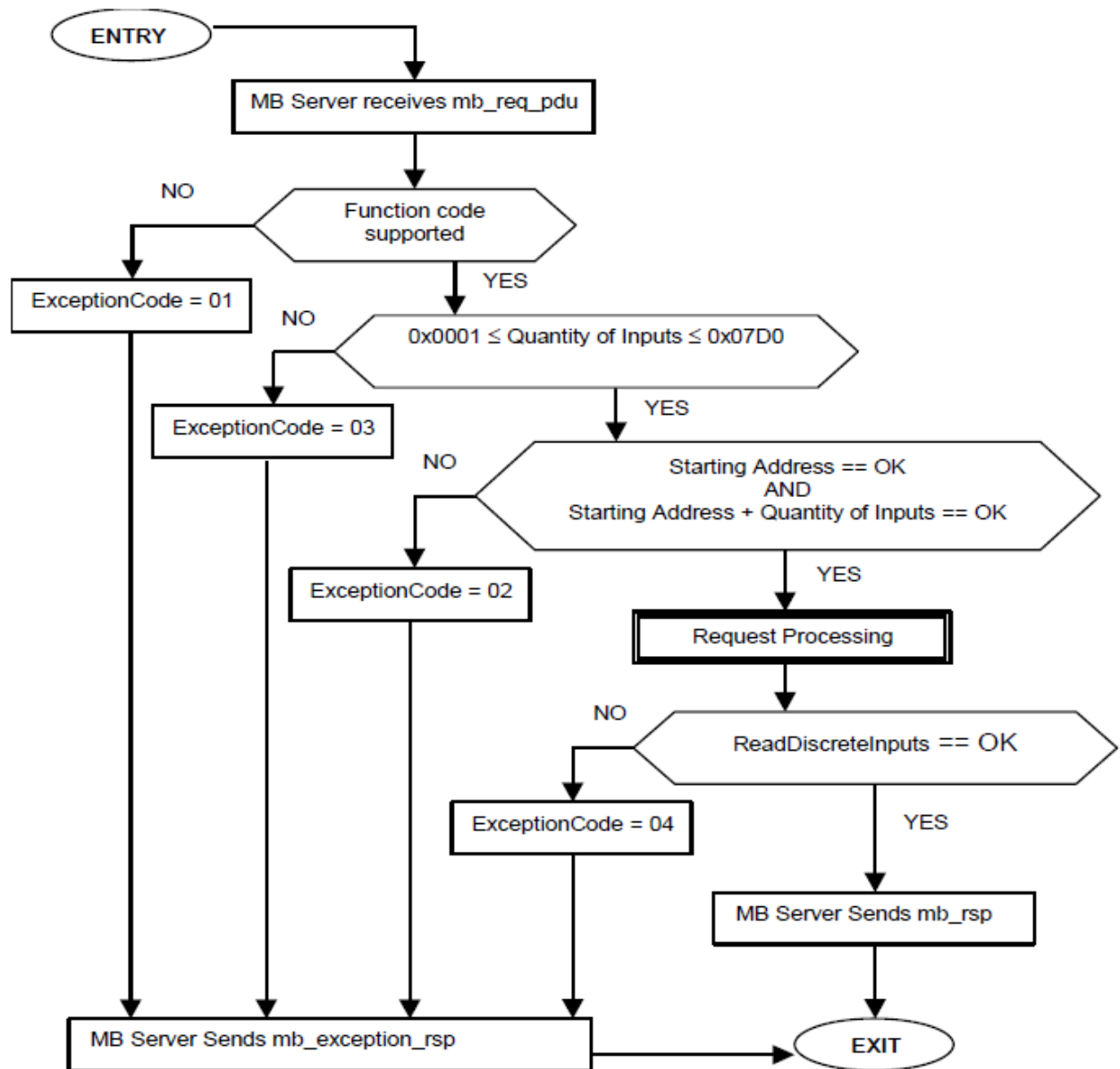
Figure 12: Read Discrete Inputs state diagram
