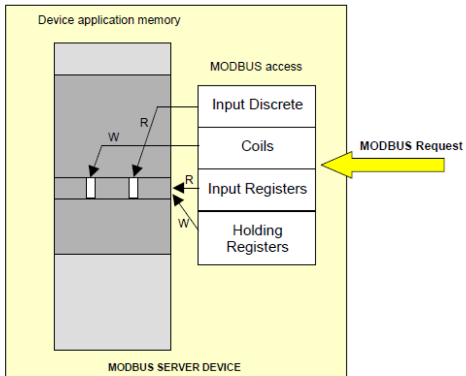
Figure 7 MODBUS Data Model with only 1 block
