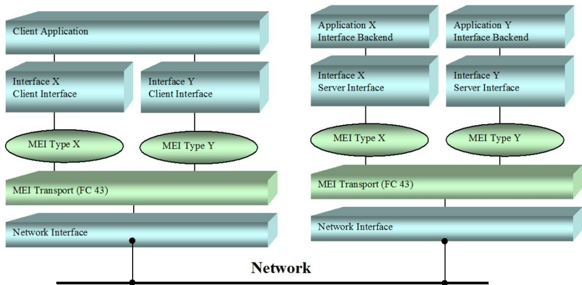
Figure 29: MODBUS encapsulated Interface Transport
