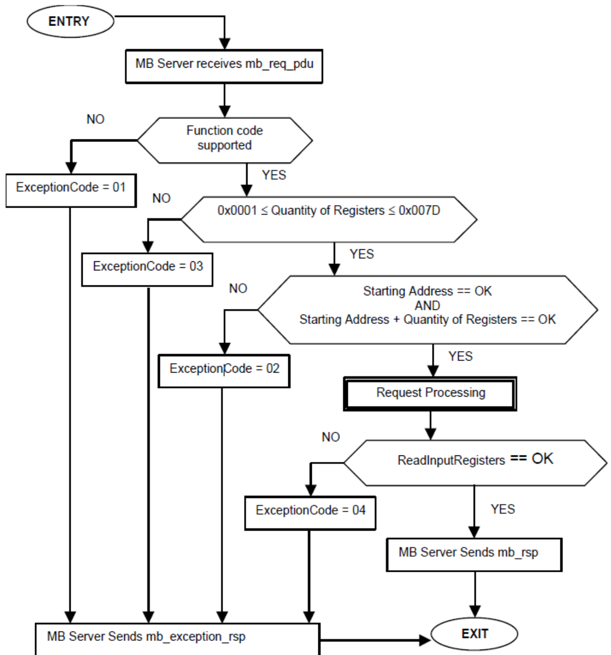
Figure 14: Read Input Registers state diagram
