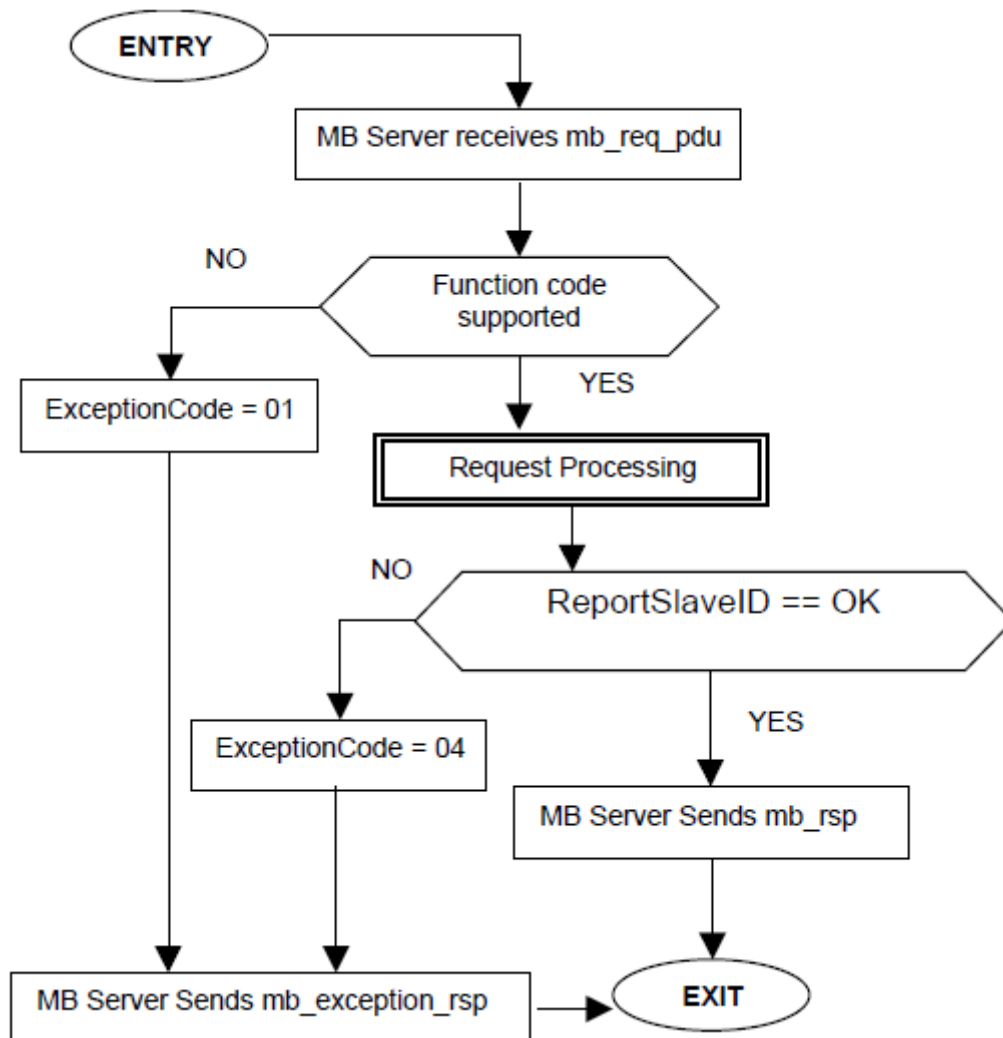
Figure 23: Report server ID state diagram
