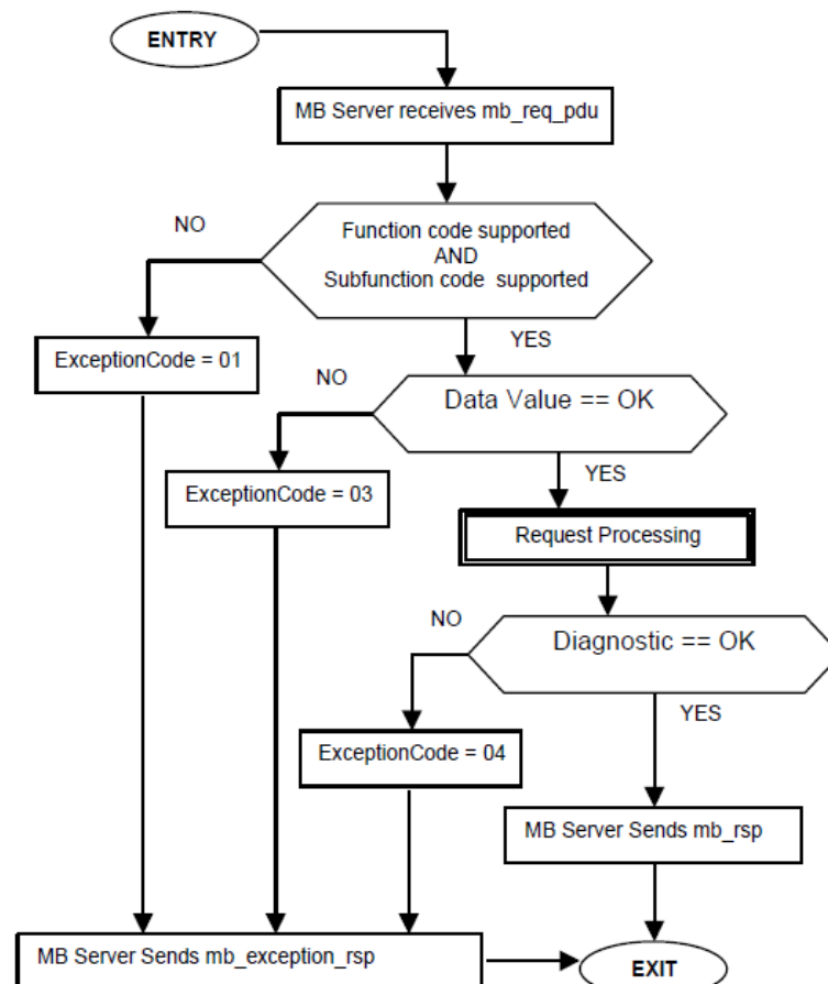
Figure 18: Diagnostic state diagram
