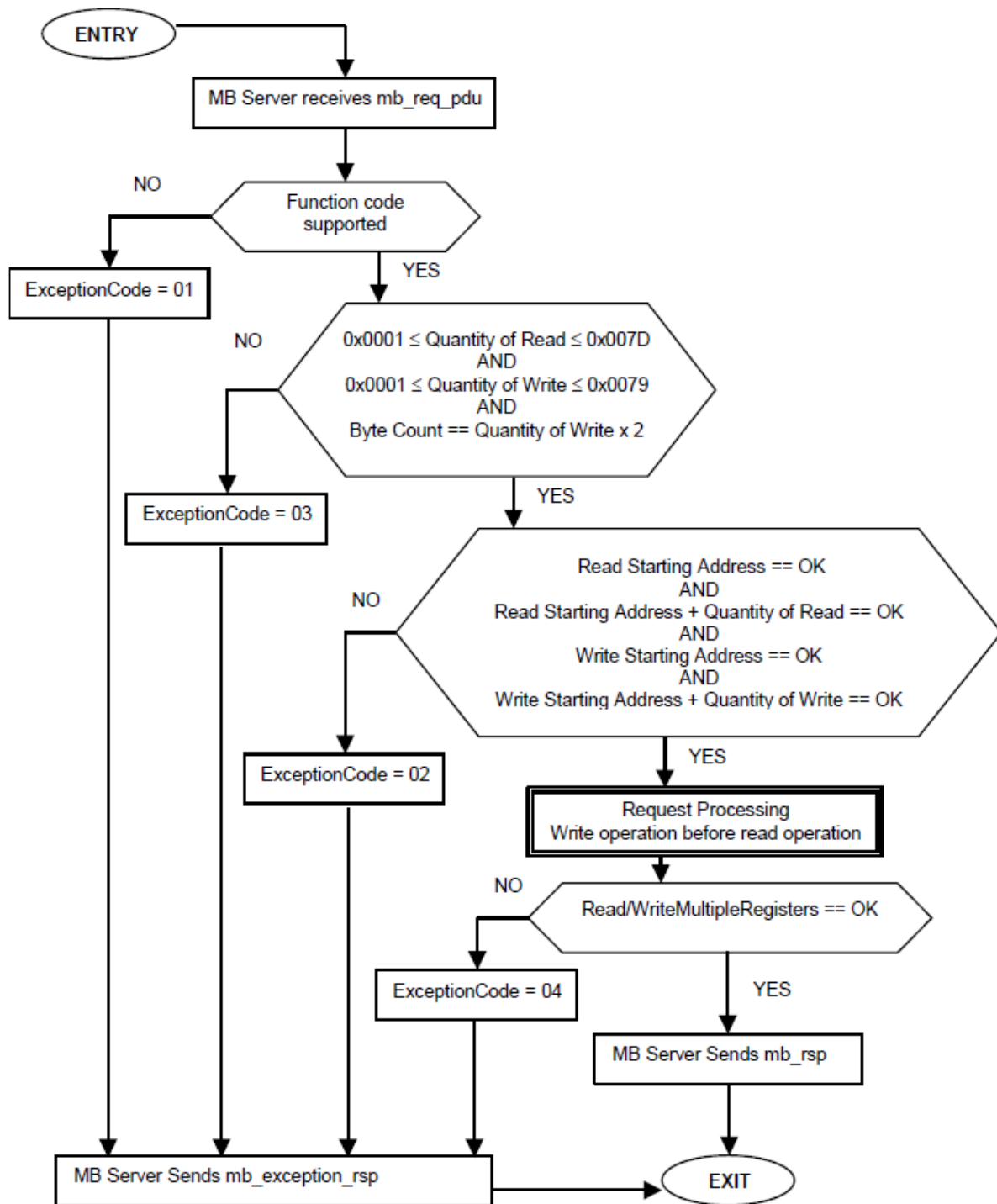
Figure 27: Read/Write Multiple Registers state diagram
