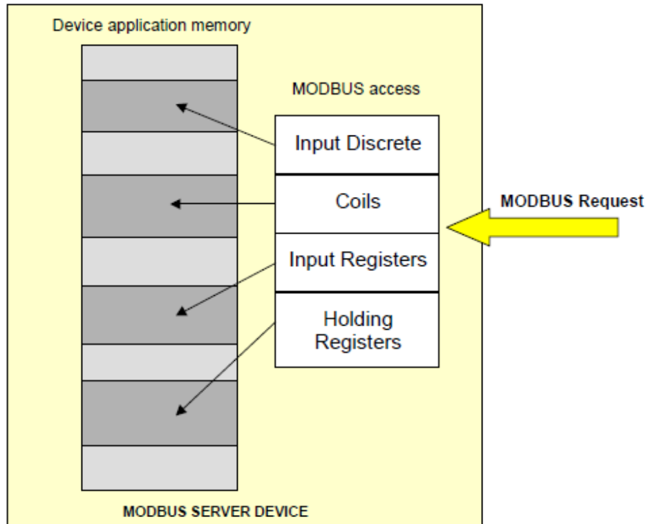
Figure 6 MODBUS Data Model with separate block
