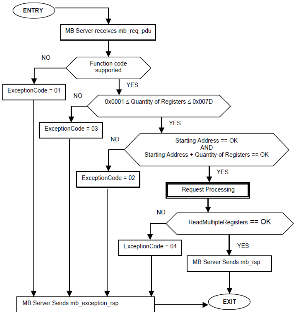
Figure 13: Read Holding Registers state diagram
