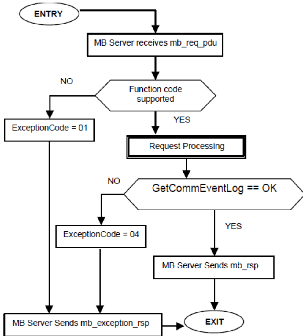
Figure 20: Get Comm Event Log state diagram
