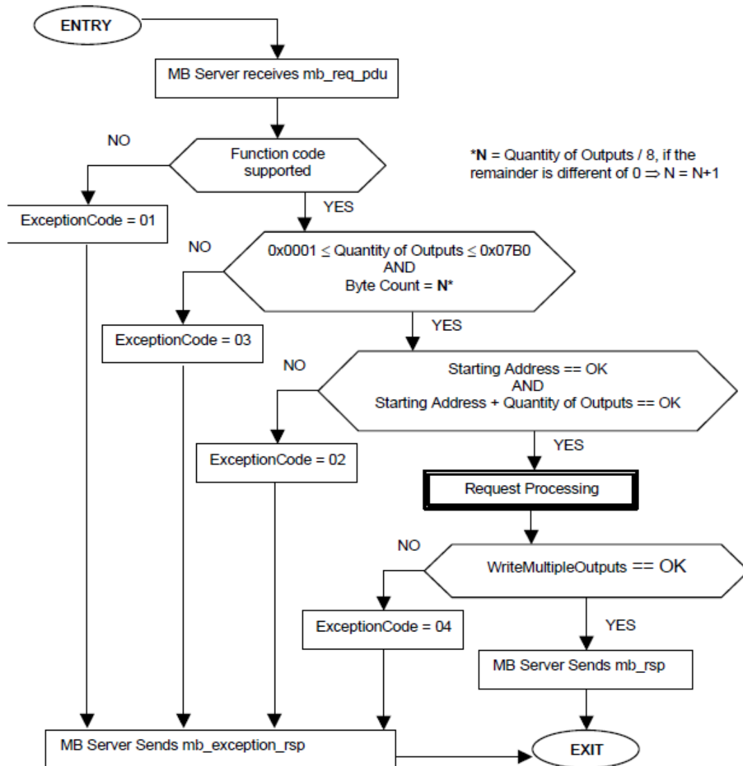
Figure 21: Write Multiple Outputs state diagram
