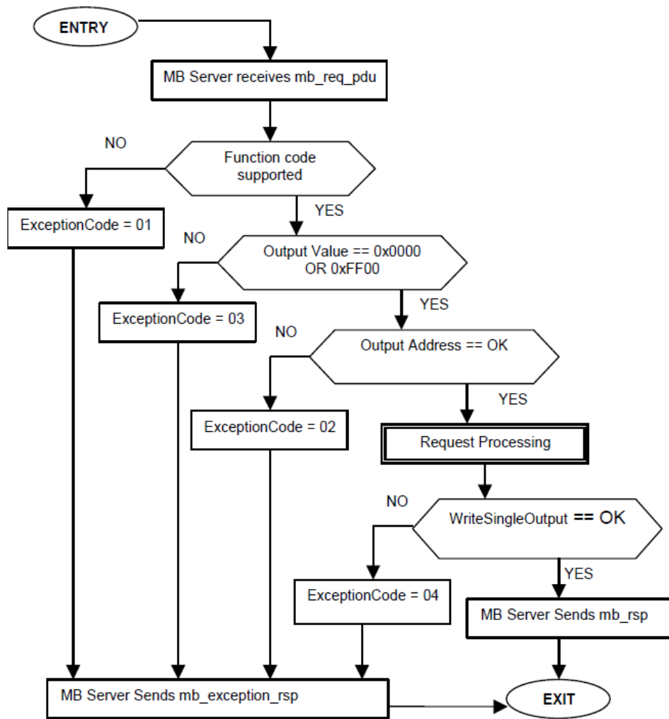
Figure 15: Write Single Output state diagram
