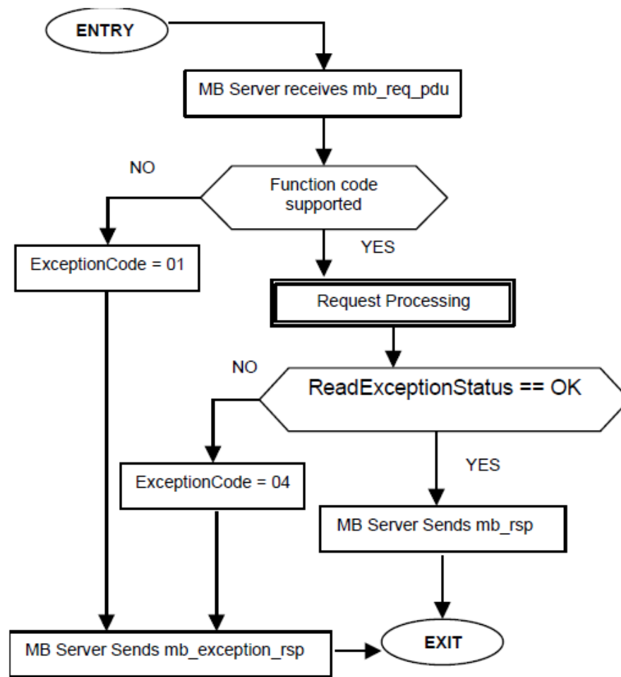
Figure 17: Read Exception Status state diagram
