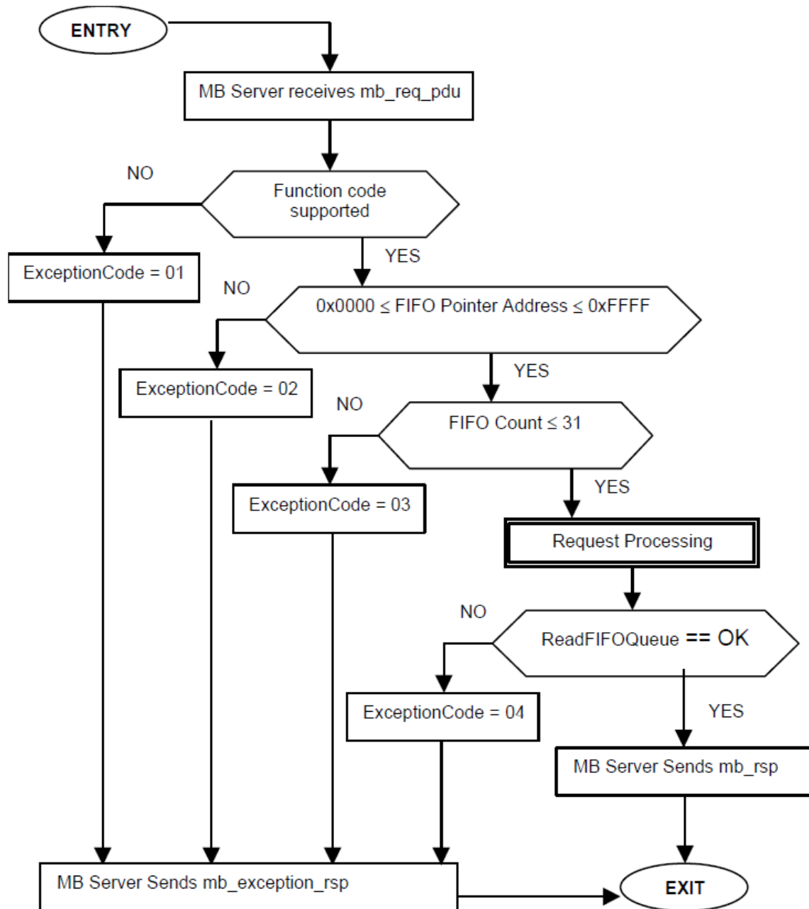
Figure 28: Read FIFO Queue state diagram
