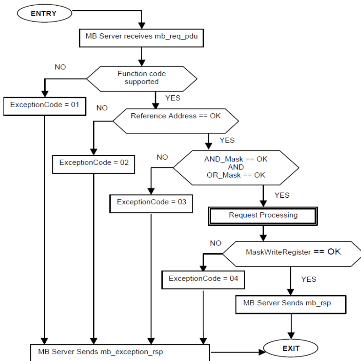
Figure 26: Mask Write Holding Register state diagram
