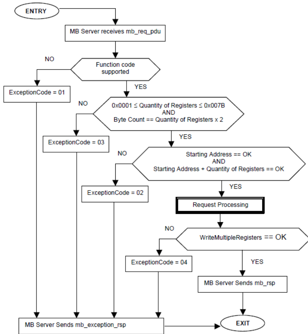
Figure 22: Write Multiple Registers state diagram
