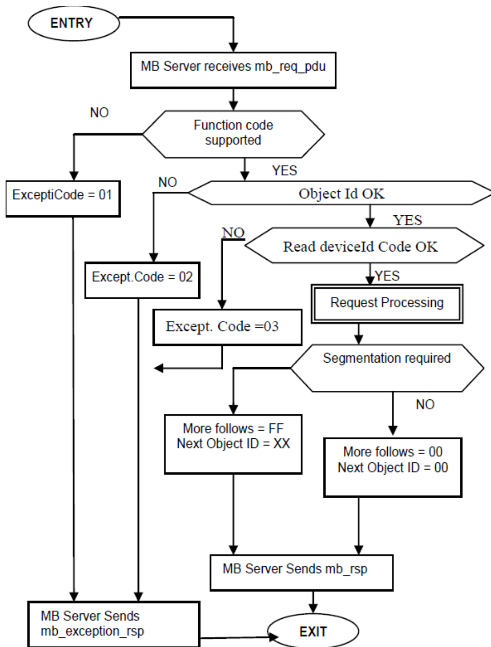
Figure 30: Read Device Identification state diagram
