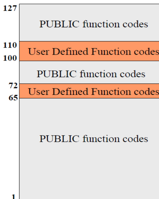
Figure 10 MODBUS Function Code Categories
