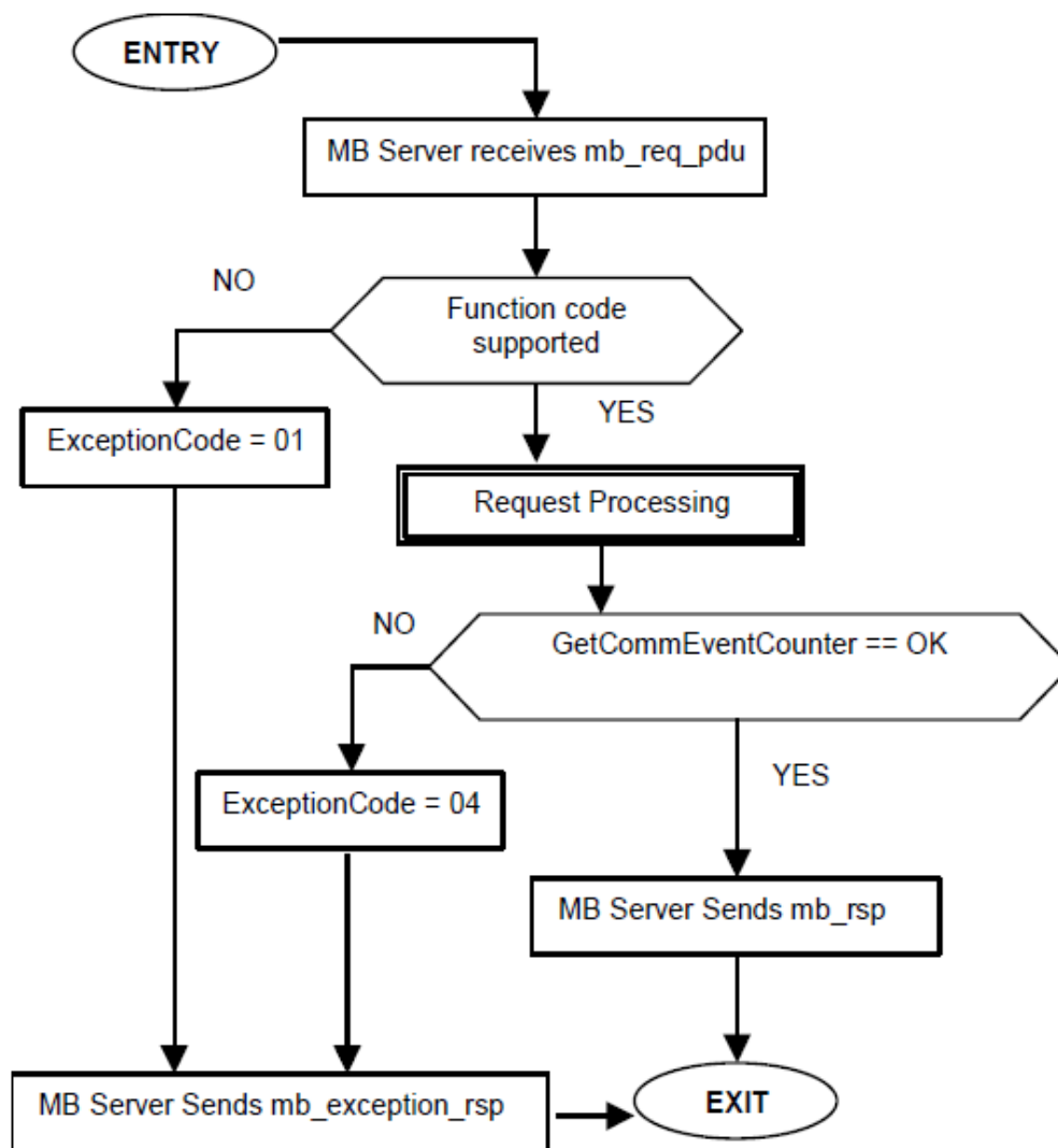
Figure 19: Get Comm Event Counter state diagram
